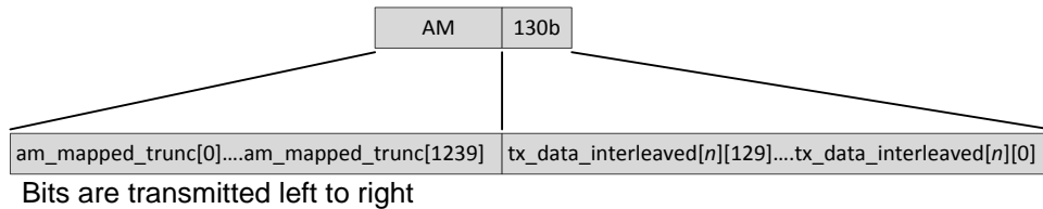
Figure 5: Alignment Marker and Data Bit Ordering
