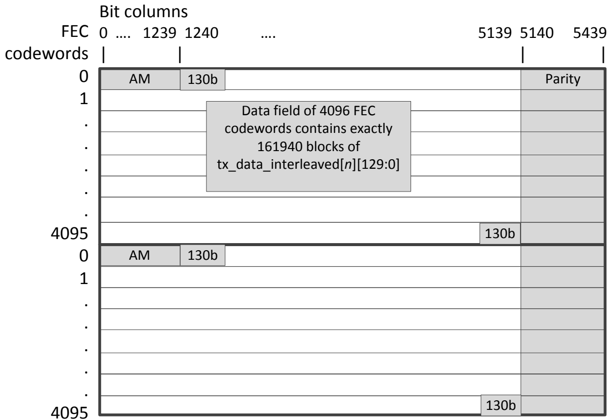
Figure 6: FEC Codewords
