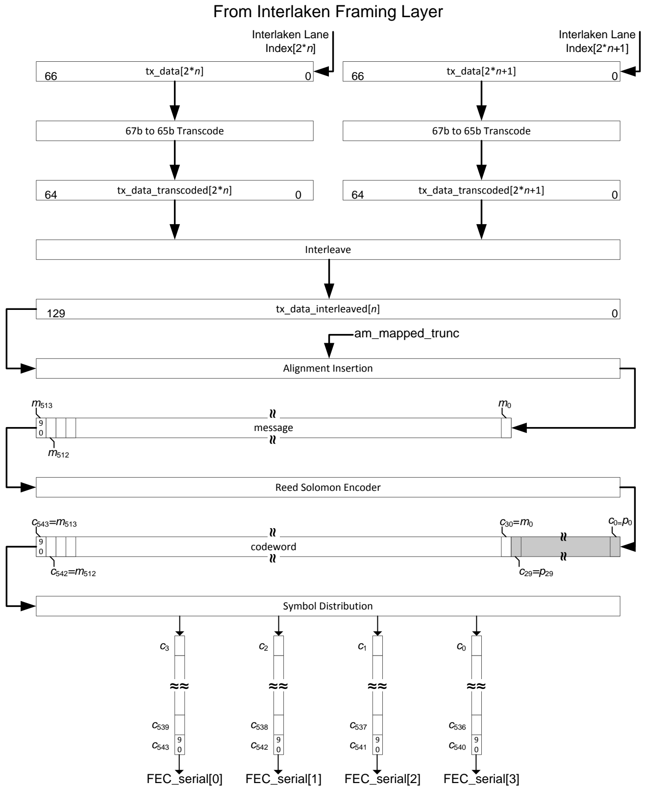
Figure 7: Transmit Bit Ordering
