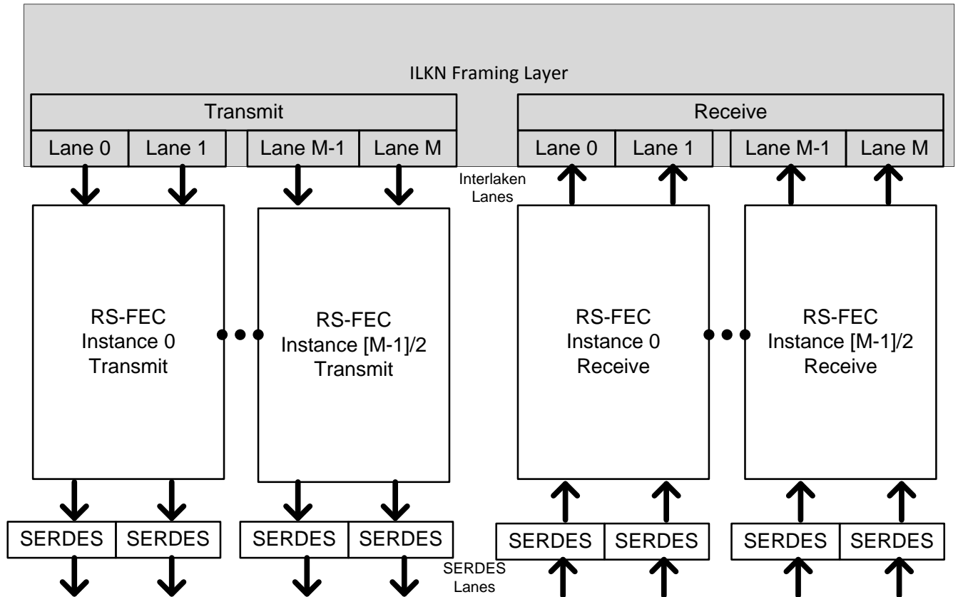
Figure 2: Overview of Interlaken Interface with RS-FEC
