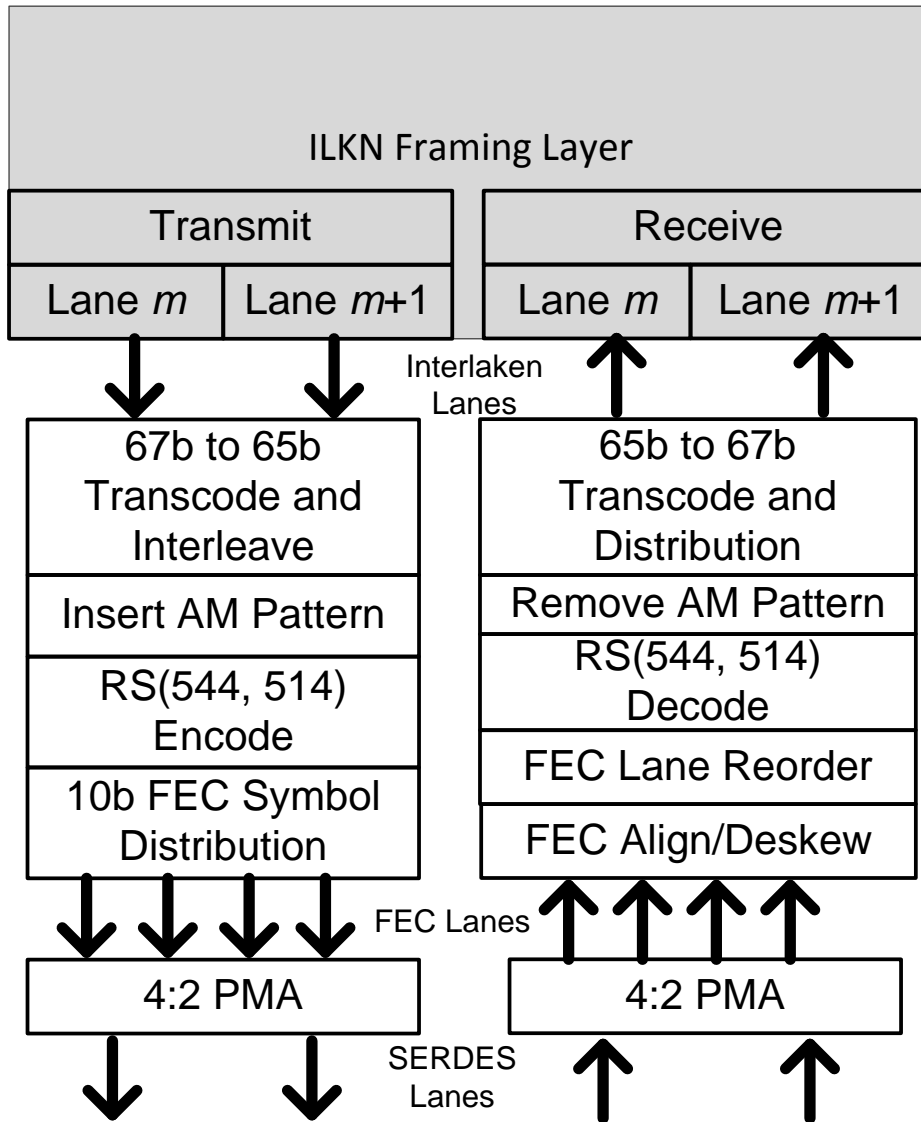
Figure 3: Detailed FEC Slice Functional Block Diagram
